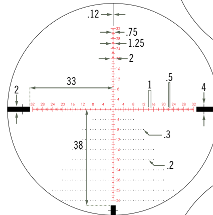
3-15 x 44 EBR-2C
