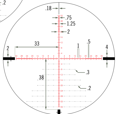
5-25 x 50 EBR-2C
