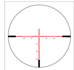
MOA Milling Hunter 2.0 Reticle
