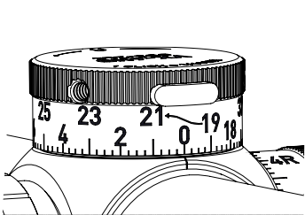
CDS-ZL2 Elevation Dial (locked position)
