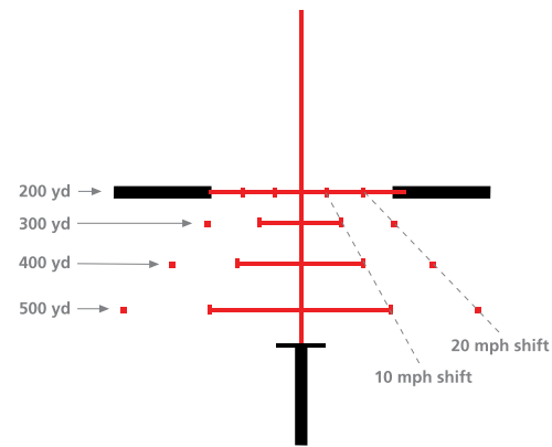
Illuminated Varmint Hunter's Reticle
