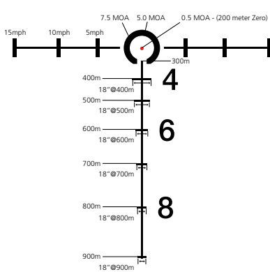
Illuminated CM-R² Reticle
