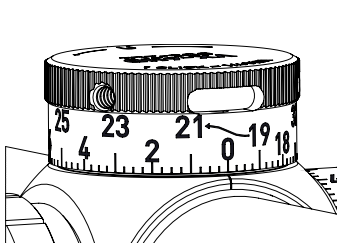
CDS-ZL2 Revolution Counter (2nd revolution)
