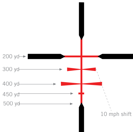
Illuminated Boone & Crockett Reticle
