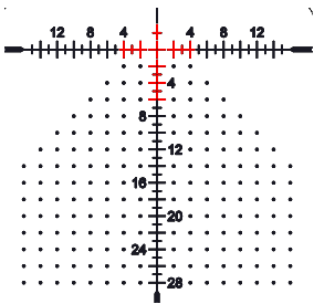
Illuminated Impact Reticle (2 MOA dot spacing and 1 MOA tick marks aid in calling bullet impact and providing aiming corrections)
