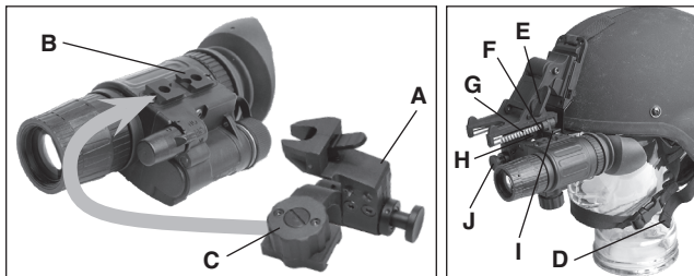
Figure 3.2 Attaching ATN NVM-14 to Helmet Mount
