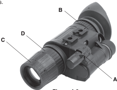
Figure 4.2 Mechanical Functions
