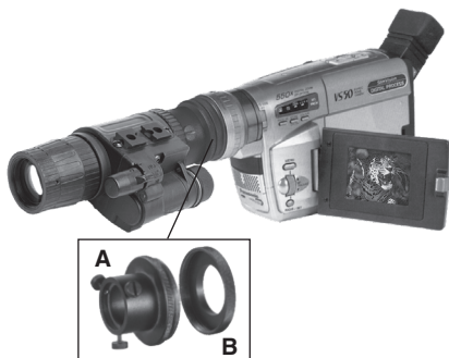
Figure 3.7 Mounting Camcorder to the ATN NVM-14
