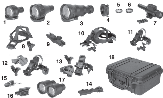
Figure 2.2 ATN NVM-14 Optional Components
