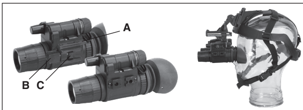
Figure 3.4 Mounting of the Dual Bridge Adapter
