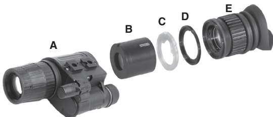
Figure 6.1 Maintenance/Replacement of the tube in the NVM-14
