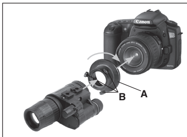
Figure 3.6 Mounting Camera to the ATN NVM-14
