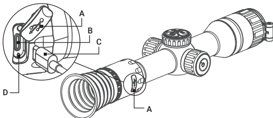
FIGURE 2-1. USB INTERFACE
